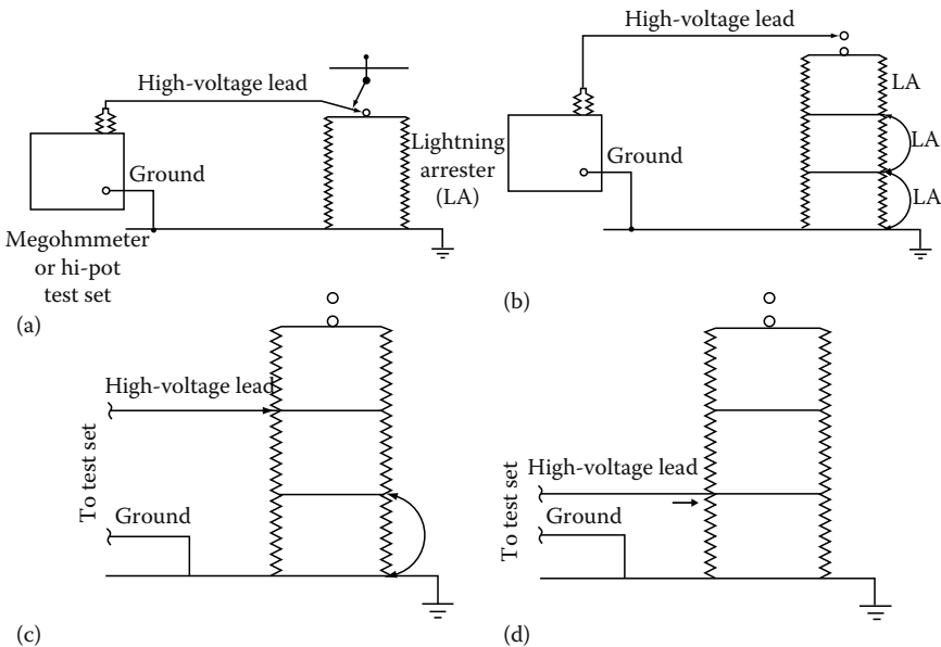
FIGURE 2.20 Lightning arrester test connections: (a) basic test connection for lightning arrester; (b) to test top arrester in stack; (c) to test middle arrester; and (d) to test bottom arrester.
