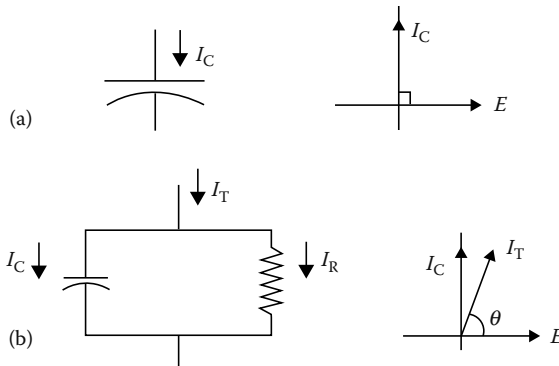
FIGURE 1.7 Electrical representation of insulation: (a) perfect and (b) practical.
