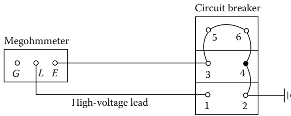
FIGURE 2.12 Typical connection for insulation resistance test of circuit breaker in open position.
