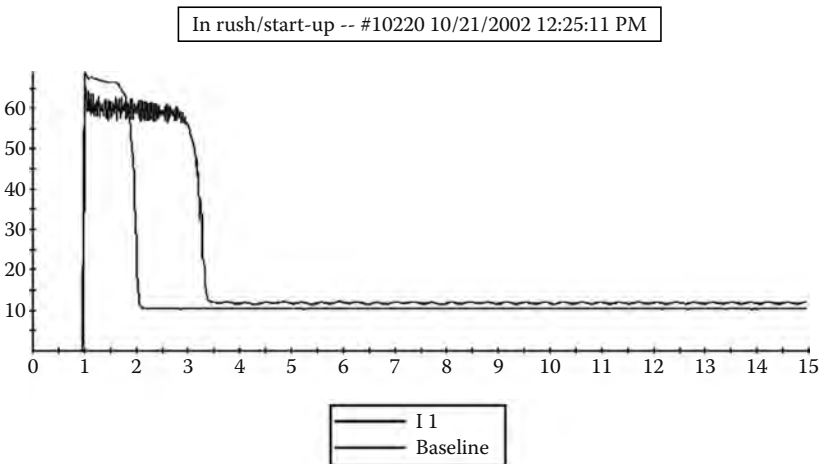
FIGURE 10.29 Graph showing inrush current of the motor relative to the baseline inrush current. (Courtesy of PdMA Corporation, Tampa, FL.)
